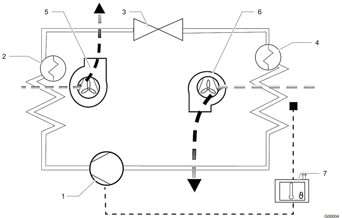
Fig. 8: Refrigeration circuit
