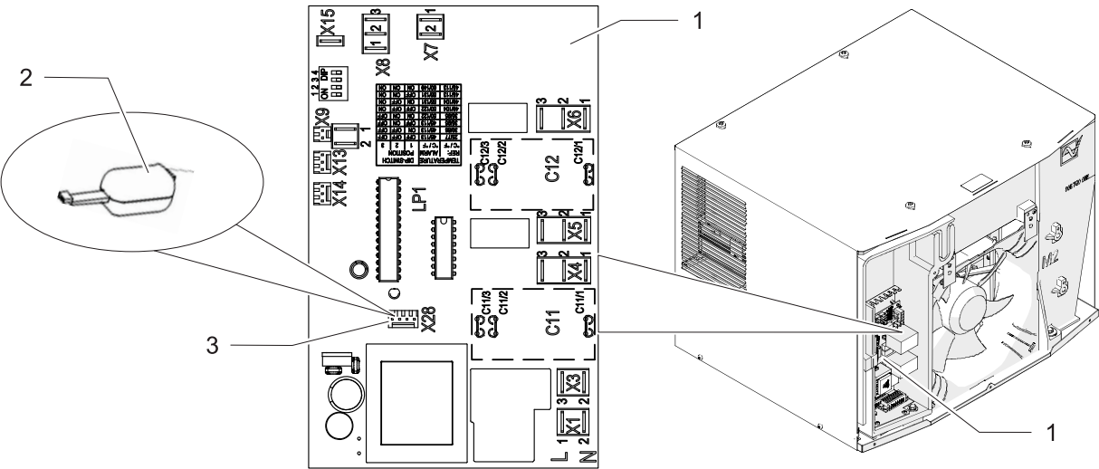
Fig. 25: Service interface
