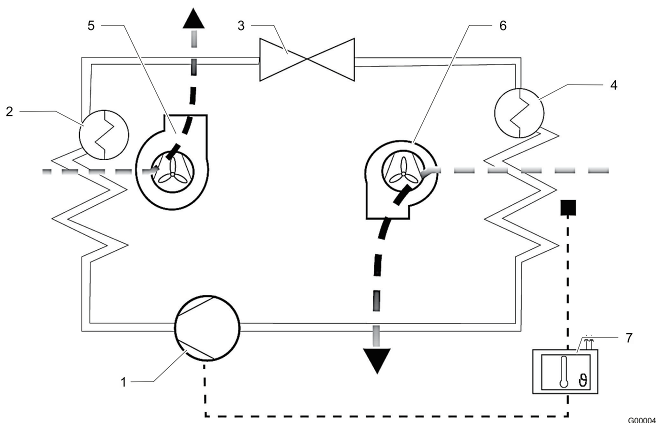
Fig. 8: circuit frigorifique
