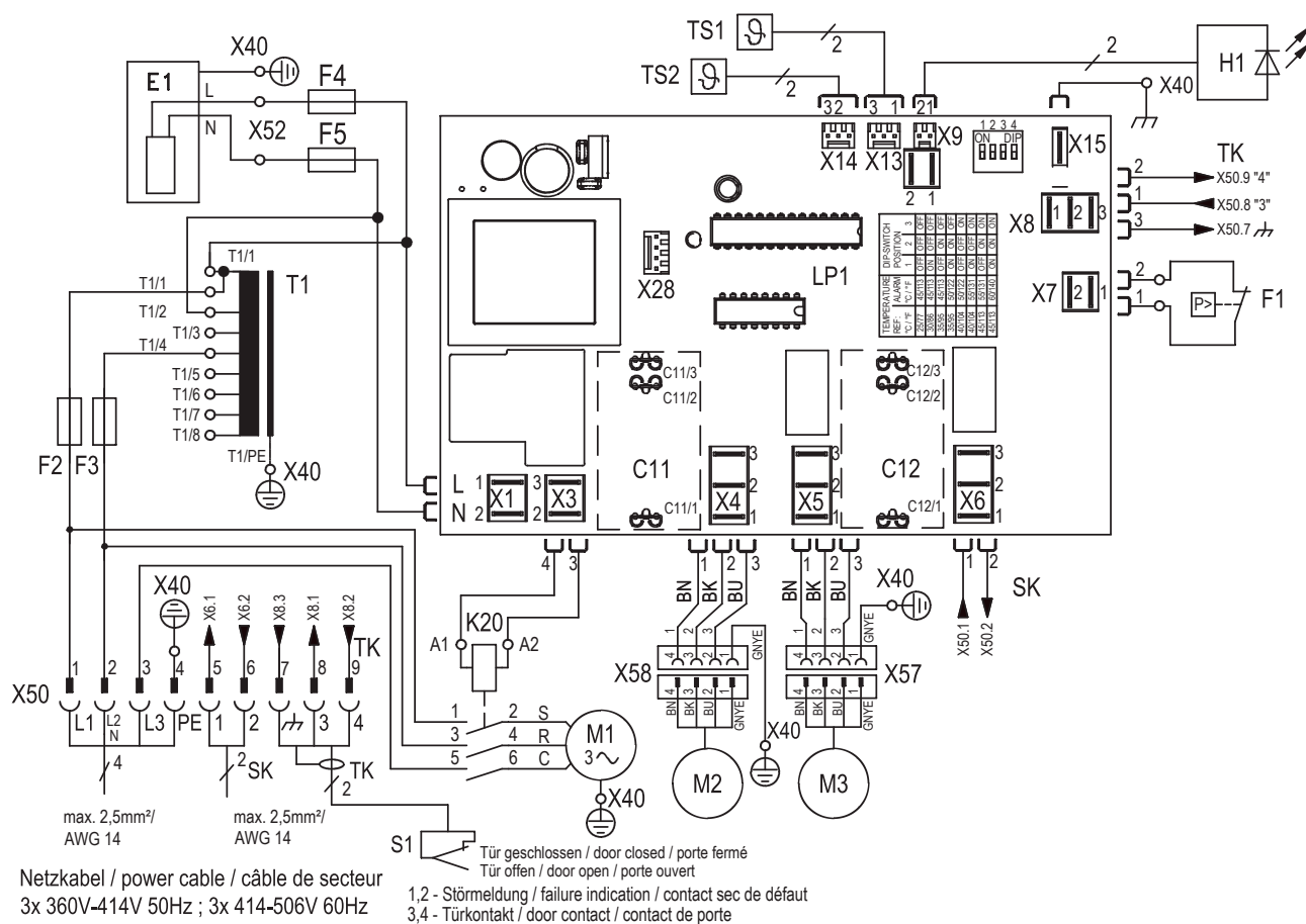
Fig. 20: Circuit diagram
