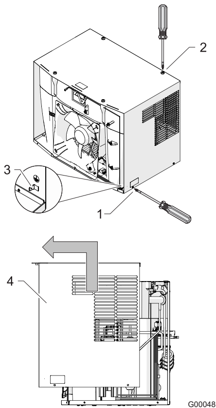
Fig. 28: Removing the front flap
