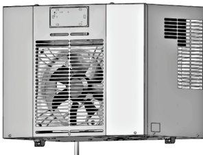
Fig. 18: Mounting the bracket
