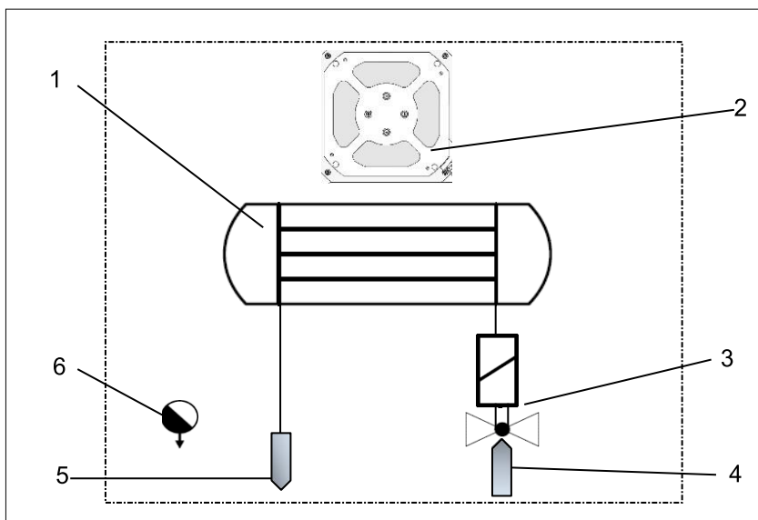
Illustration 3 - Cycle frigorifique
