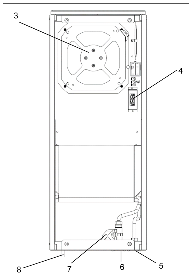
Figure 1 – Interior view Air/ water heat exchanger
