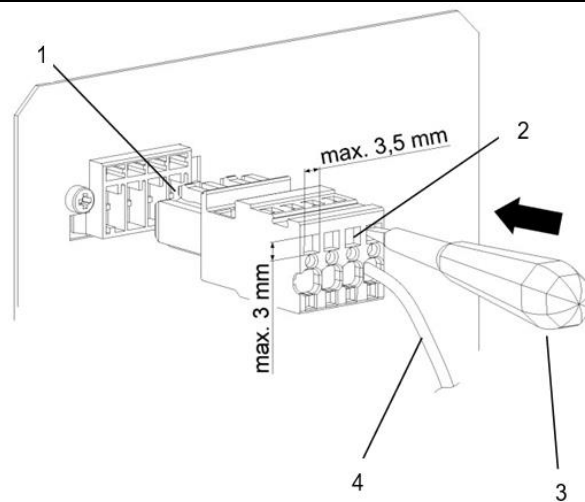
Figure 16 - Plug connection for air/water heat exchanger
