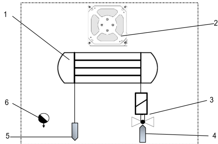
Figure 3 - Refrigerant circuit
