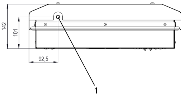
Figure 13 – Condensate drain connection PWI
