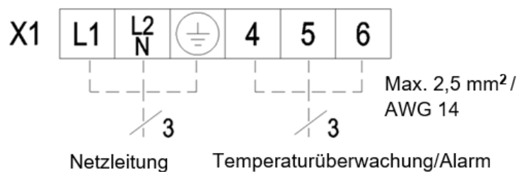
Figure 15 – Electrical connection
