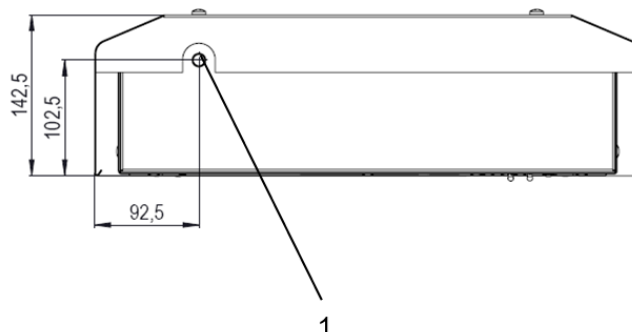
Illustration 14 – Raccordement de l'évacuation du condensat PWS
