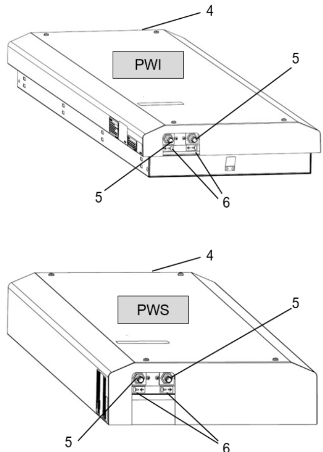
Figure 12 – Cooling water connections with threaded hose nozzles (top view)
