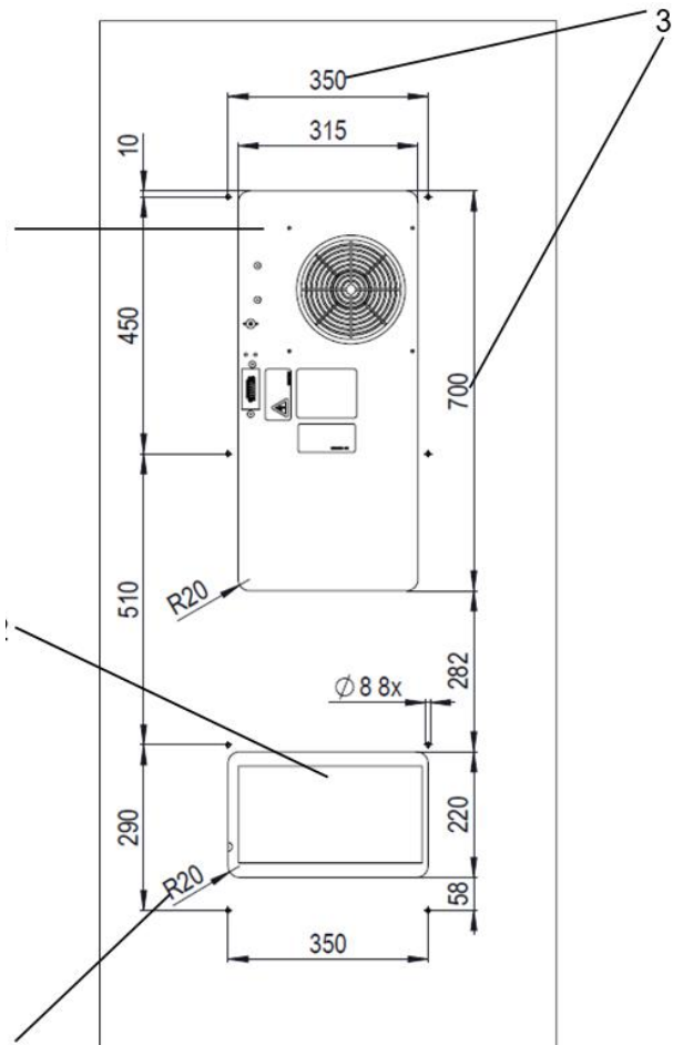
Figure 6 - Switch cabinet exterior view Cut-out for PWS air/water heat exchangers
