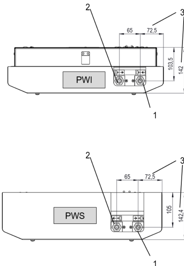
Figure 11 – Cooling water connections Water outlet/ water inlet (top view)
