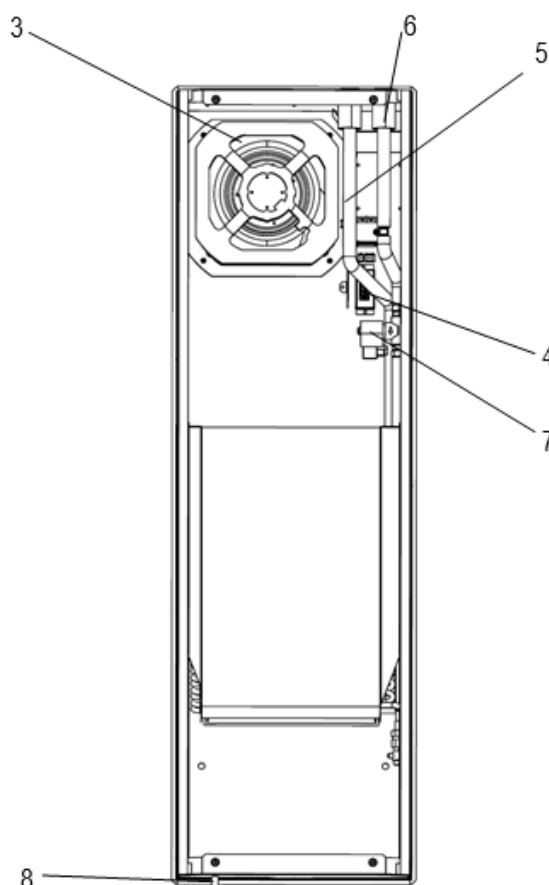
Figure 2 – Interior view Air/ water heat exchanger
