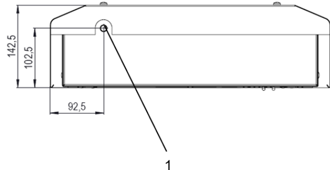
Figure 14 – Condensate drain connection PWS
