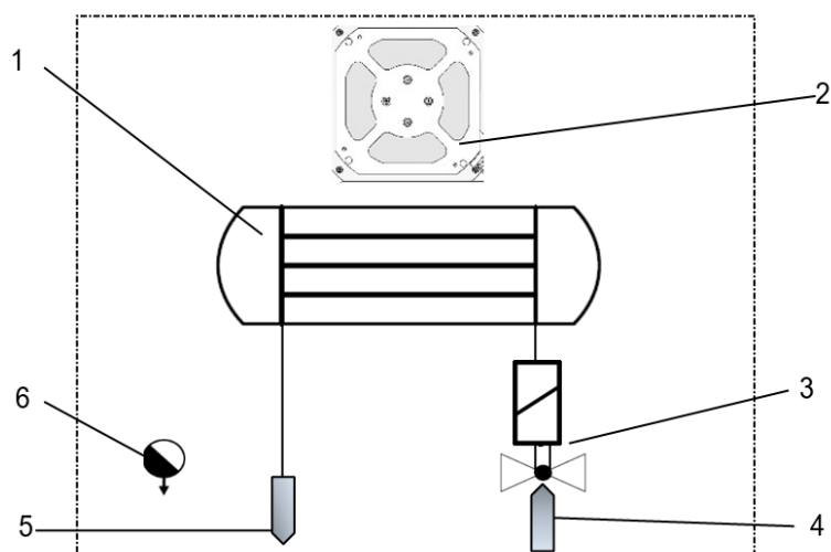
Illustration 3 - Cycle frigorifique
